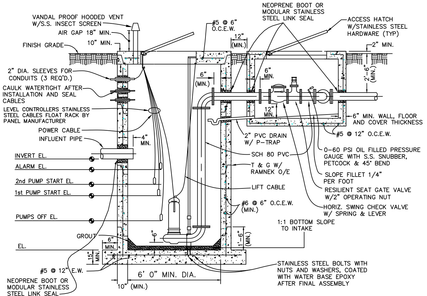
SECTION VIEW
