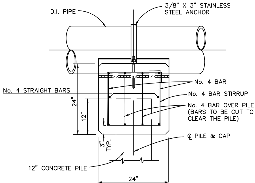
VIEW C-C
