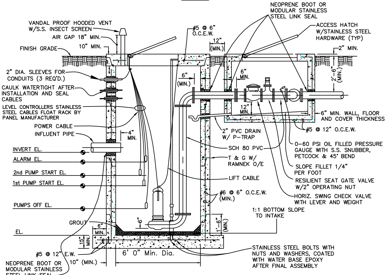
TYPICAL LIFT STATION DETAIL
